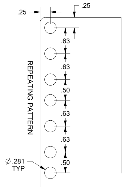
DETAIL A NOT TO SCALE
