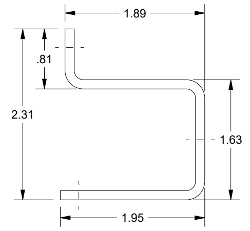
BEND DETAIL NOT TO SCALE
