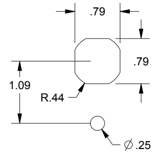
CUTOUT DETAIL
