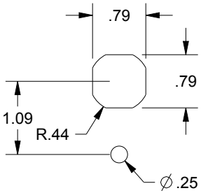
CUTOUT DETAIL
