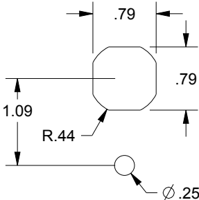
CUTOUT DETAIL
