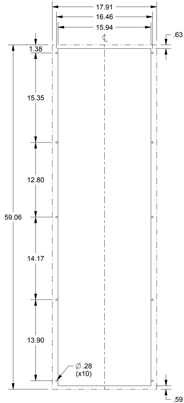
CUTOUT FOR INTERNAL INSTALLATION
