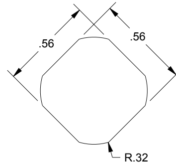
CUTOUT DETAIL
