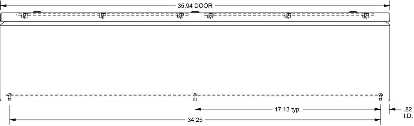
BOTTOM VIEW
