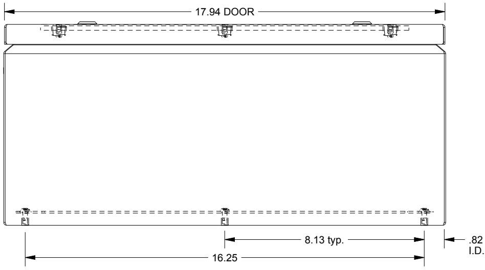
BOTTOM VIEW
