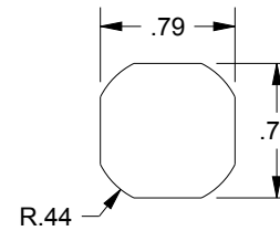
CUTOUT DETAIL
