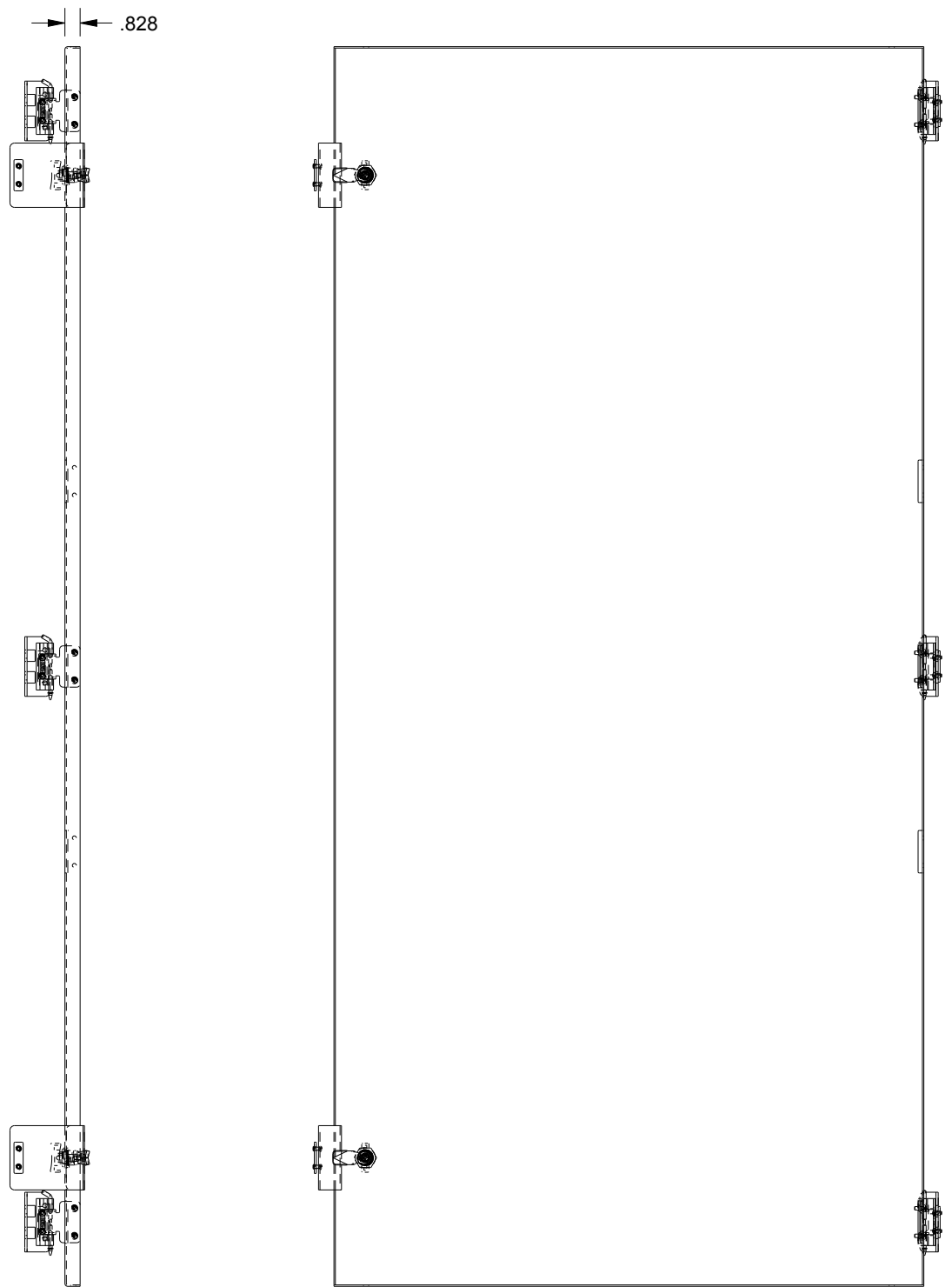
DEAD FRONT PANEL REAR VIEW
