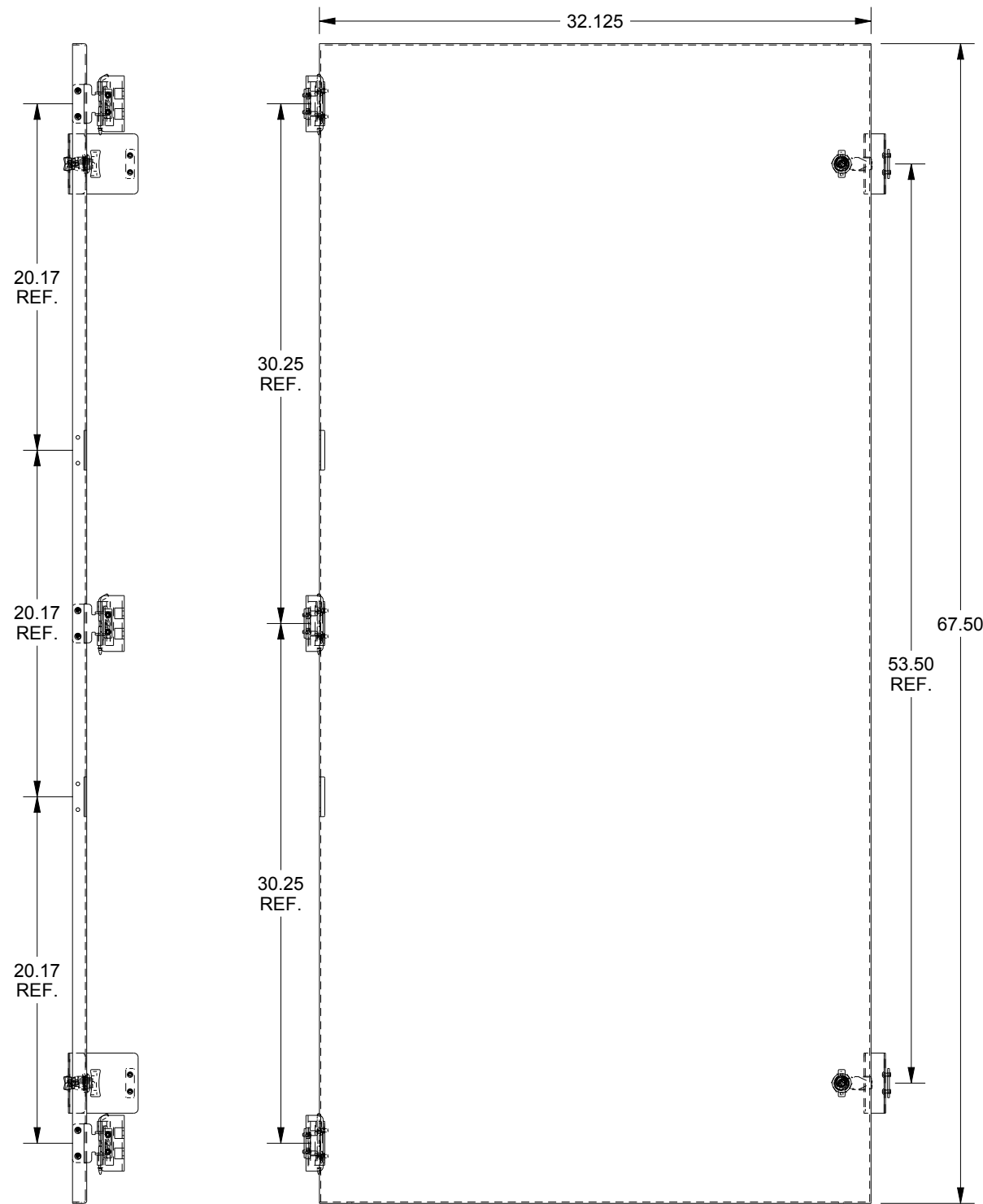
DEAD FRONT PANEL FRONT VIEW
