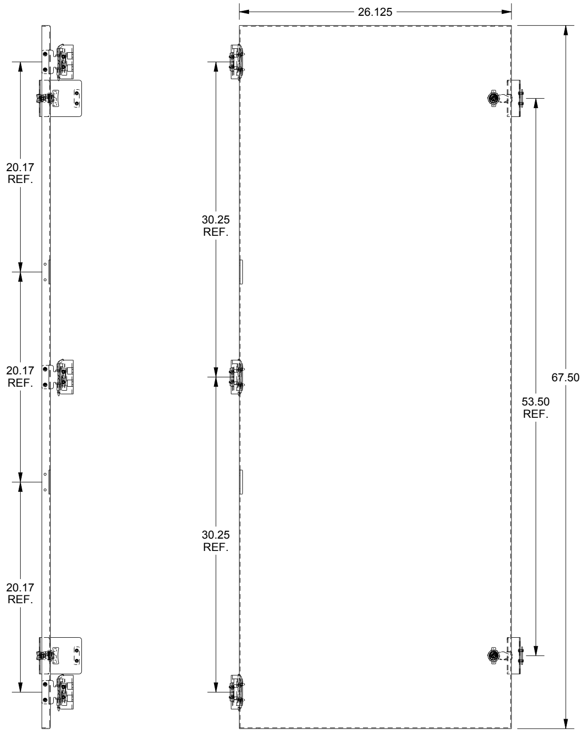
DEAD FRONT PANEL FRONT VIEW
