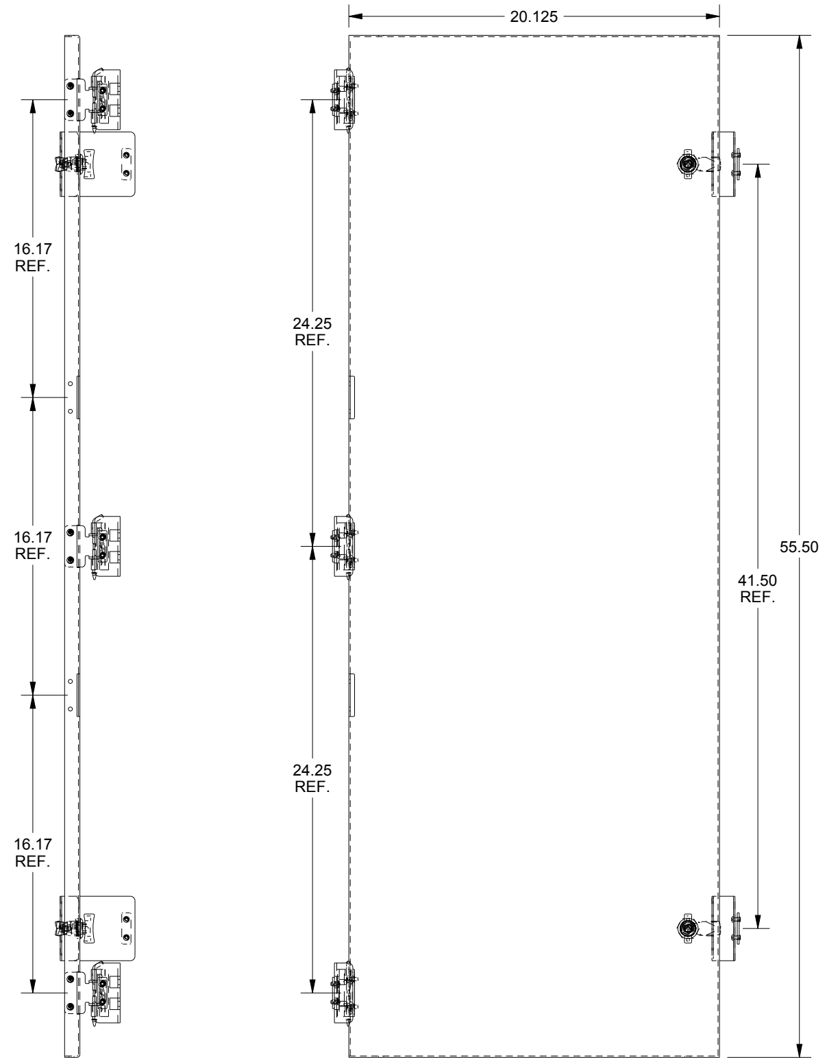
DEAD FRONT PANEL FRONT VIEW
