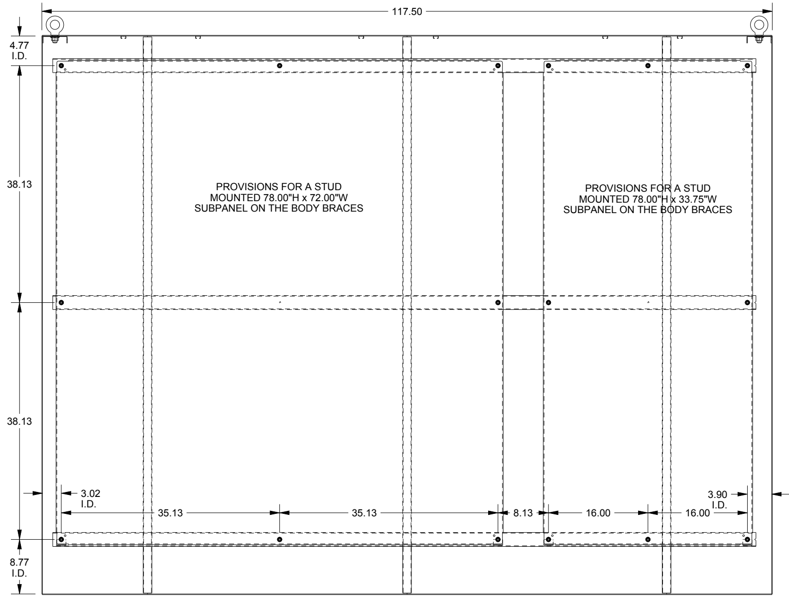
SECTION X-X
