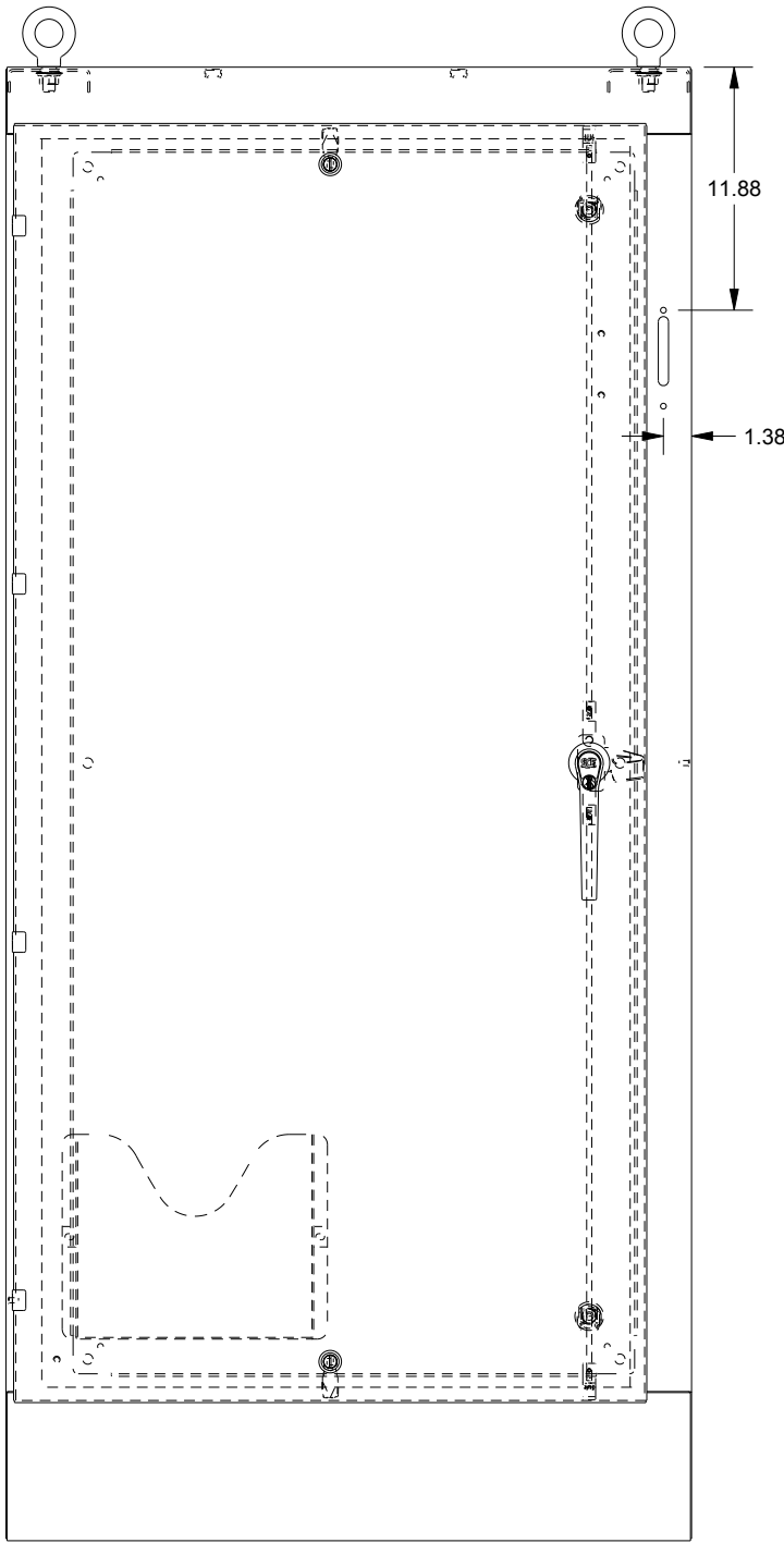
FRONT VIEW
