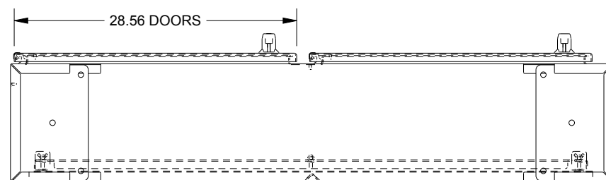
BOTTOM VIEW
