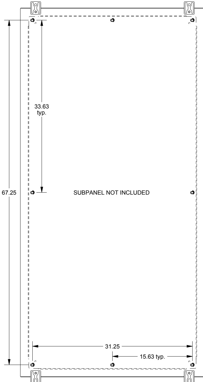
EXTERNAL REAR VIEW
