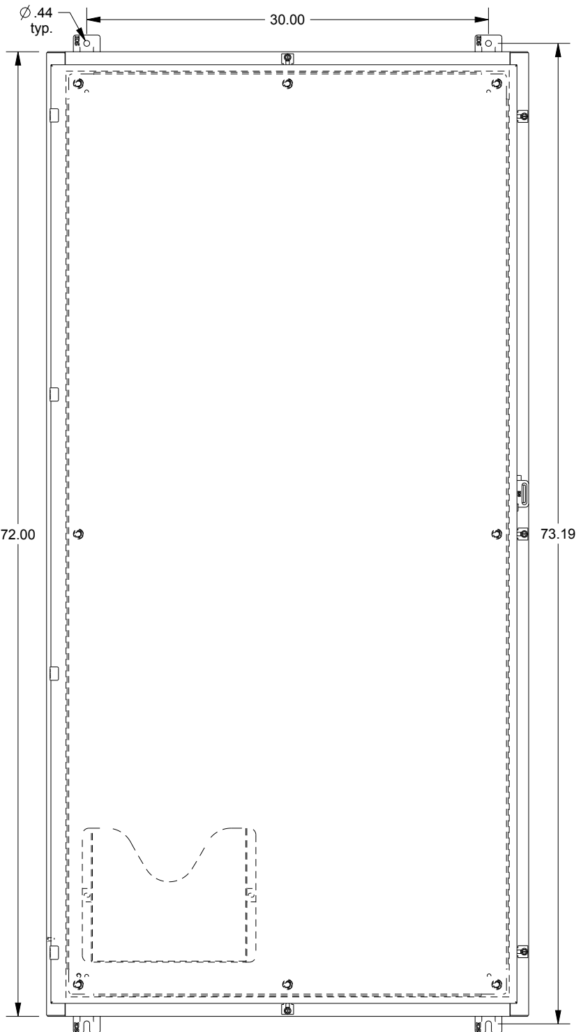
FRONT VIEW
