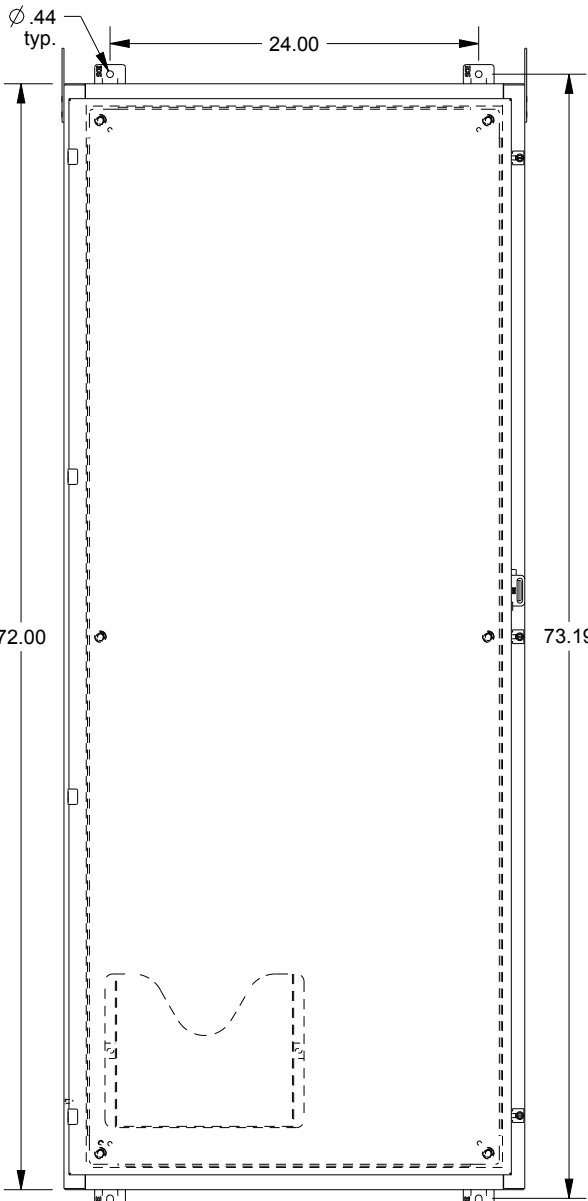
FRONT VIEW
