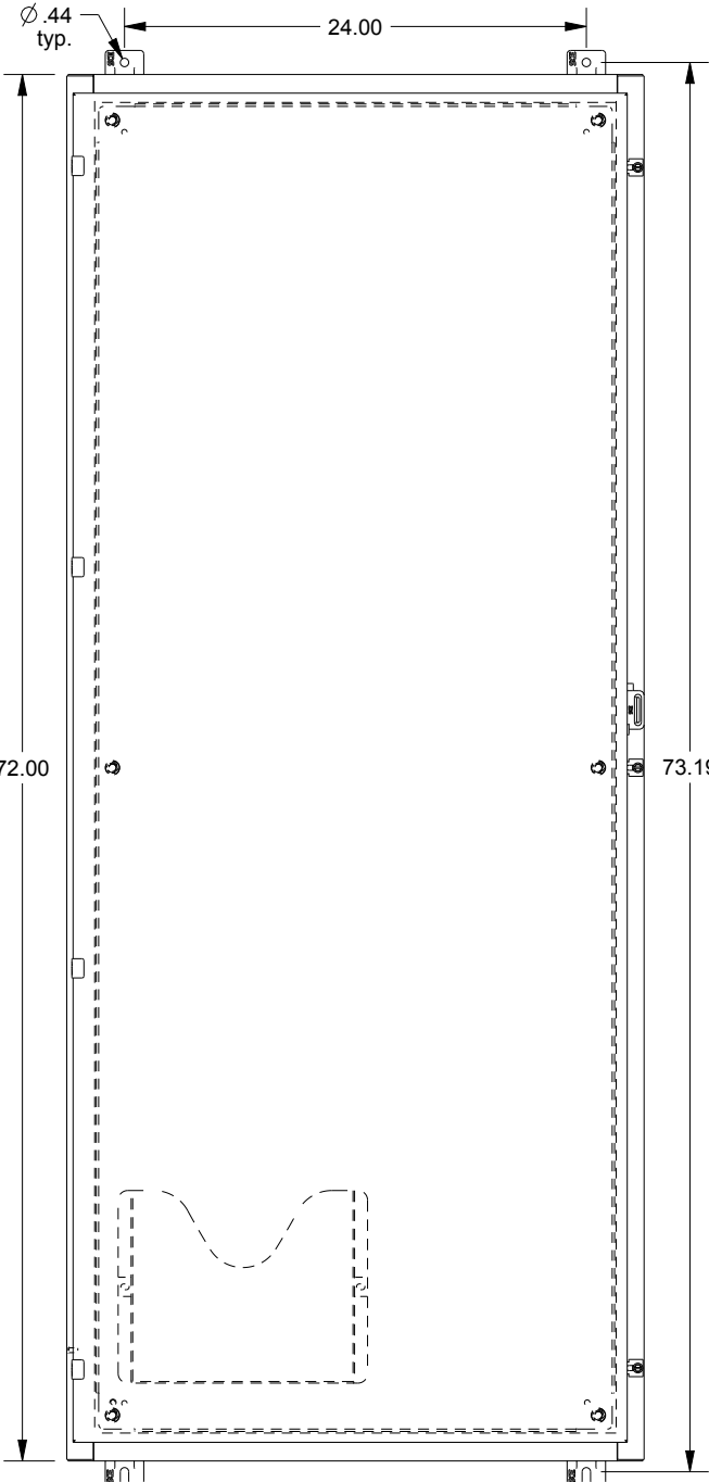
FRONT VIEW
