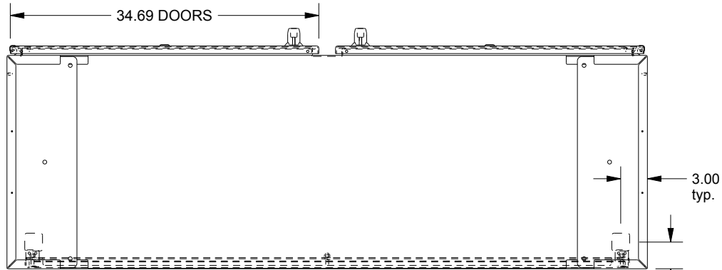
BOTTOM VIEW
