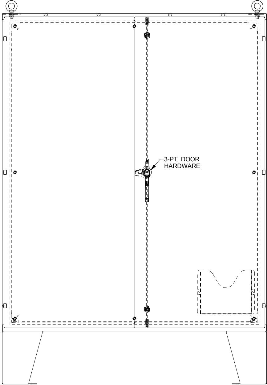
FRONT VIEW
