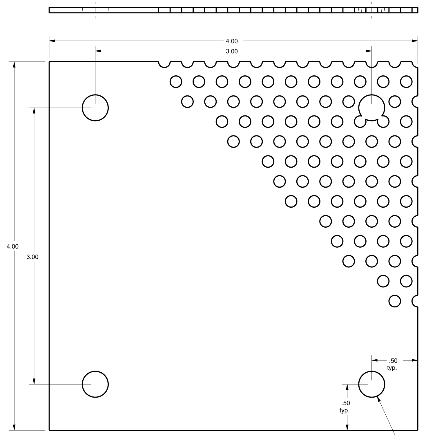
SUBPANEL FRONT VIEW
