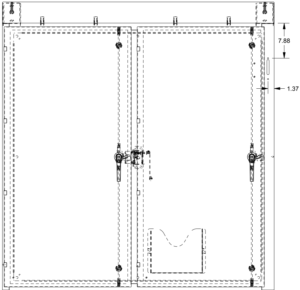
FRONT VIEW
