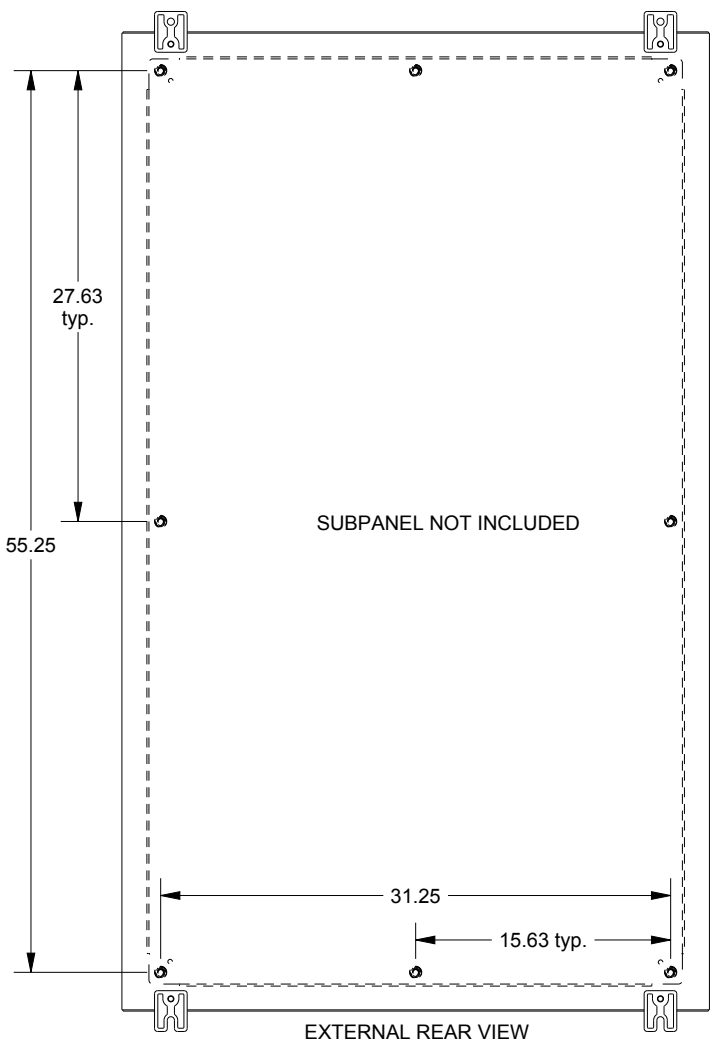
EXTERNAL REAR VIEW
