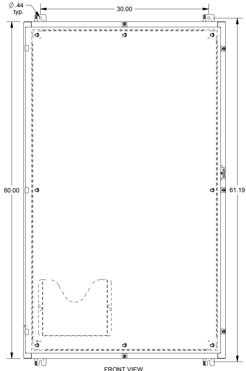
FRONT VIEW
