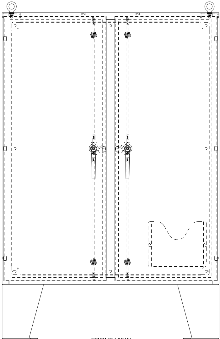
FRONT VIEW
