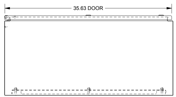
BOTTOM VIEW
