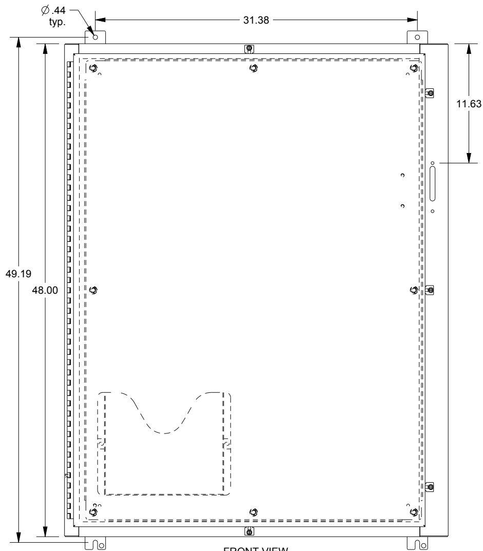
FRONT VIEW
