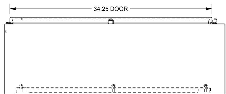
BOTTOM VIEW
