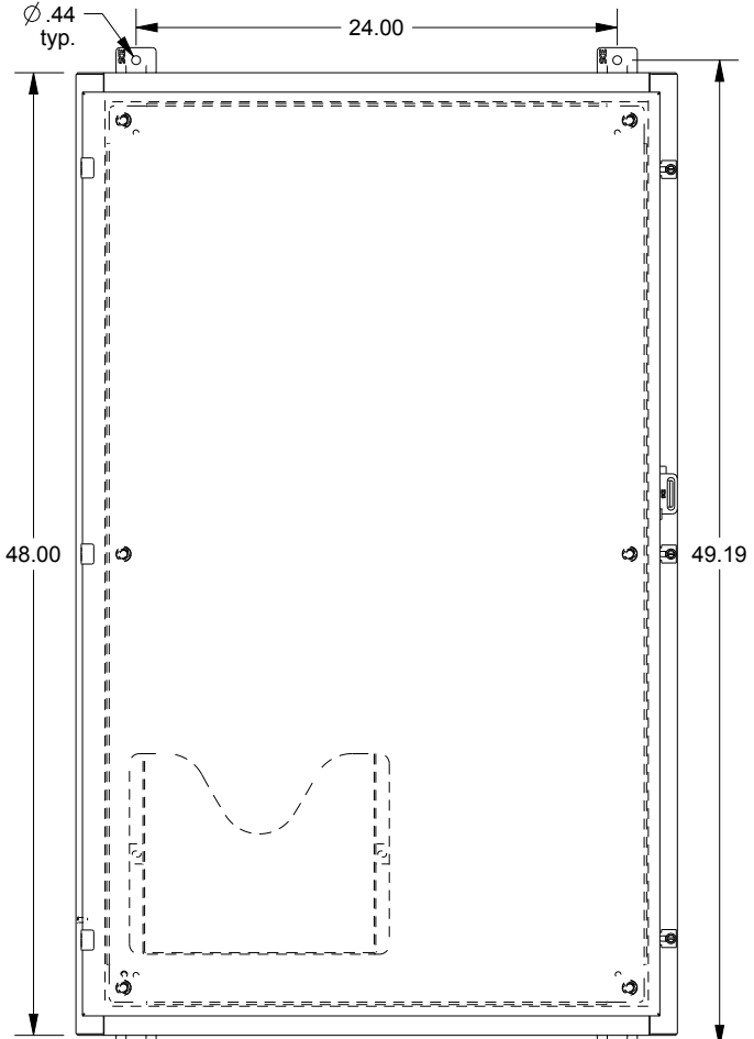
FRONT VIEW
