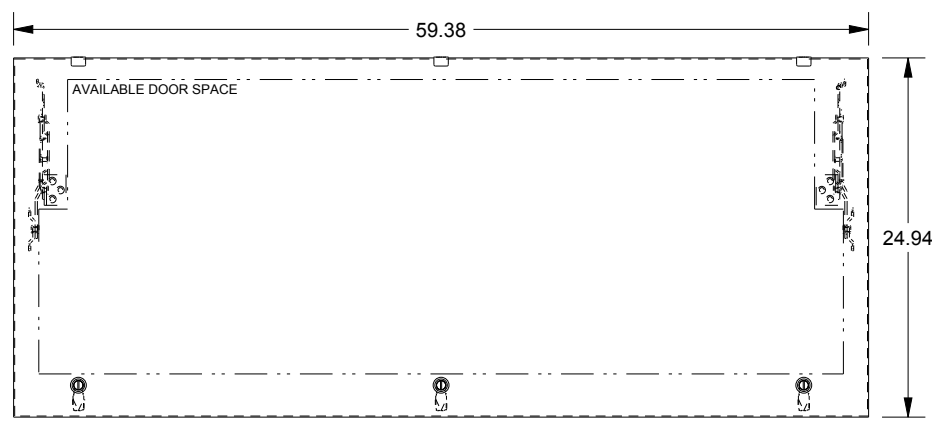
SLOPE DOOR DETAIL
