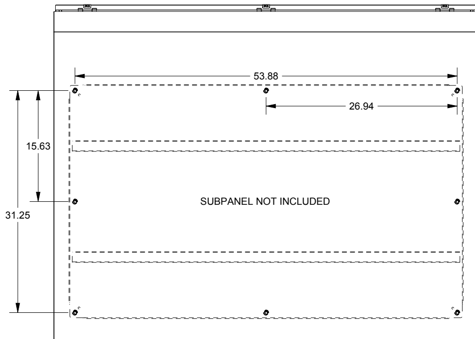
EXTERNAL REAR VIEW
