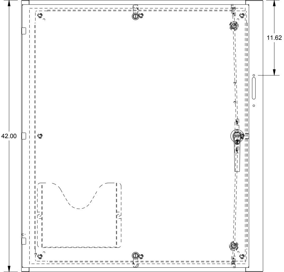
FRONT VIEW
