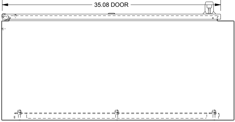
BOTTOM VIEW
