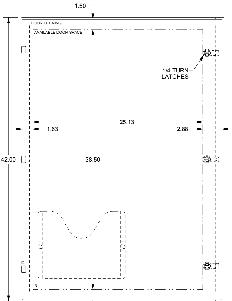
FRONT VIEW
