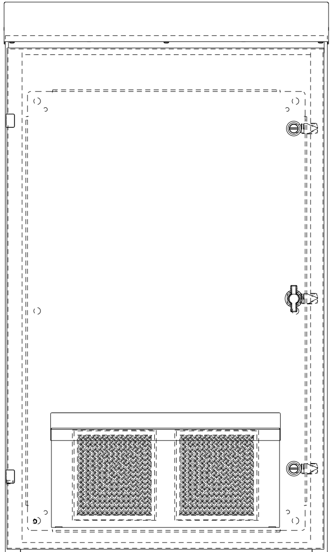
FRONT VIEW
