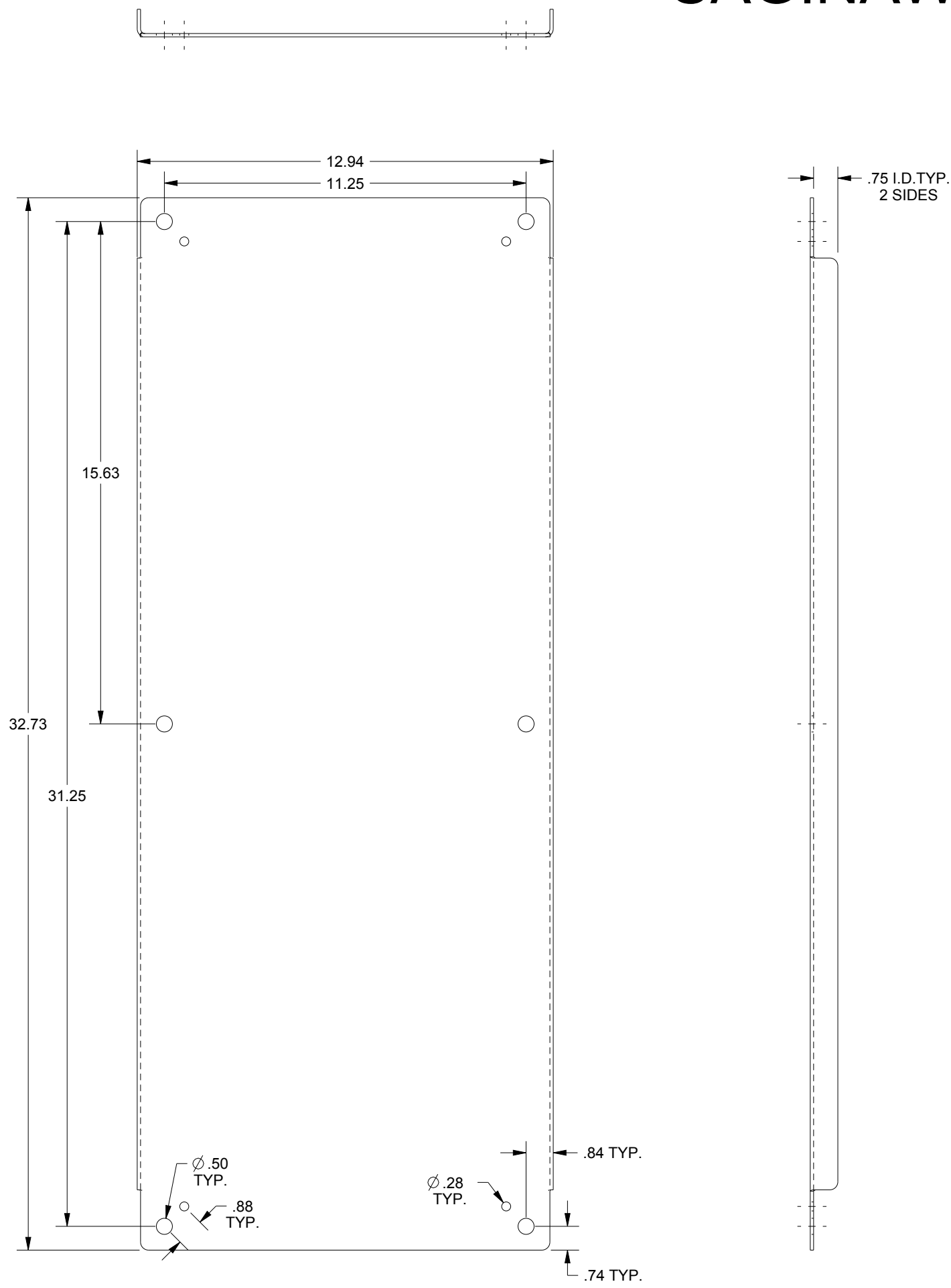
SUBPANEL FRONT VIEW
