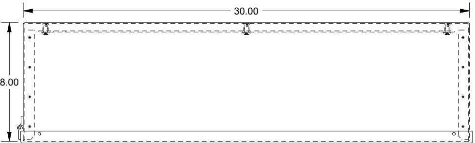
TOP VIEW
