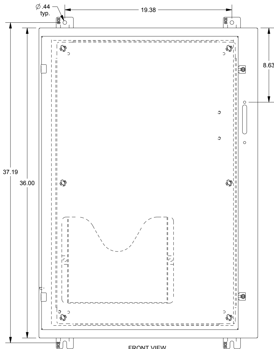
FRONT VIEW
