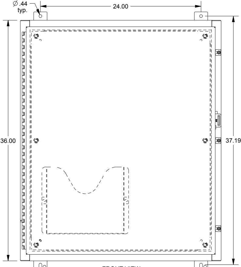
FRONT VIEW
