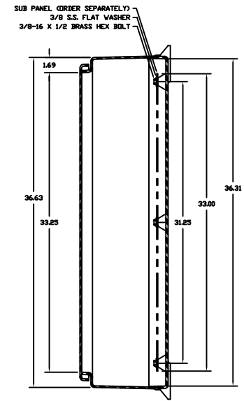
SECTION B-B
