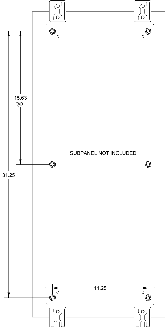
EXTERNAL REAR VIEW
