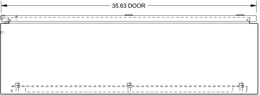
BOTTOM VIEW
