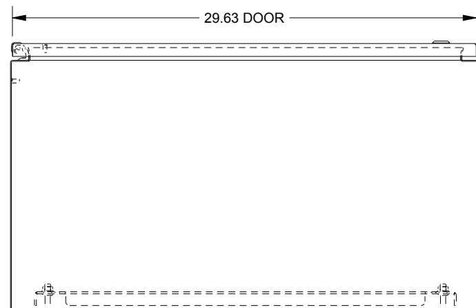
BOTTOM VIEW
