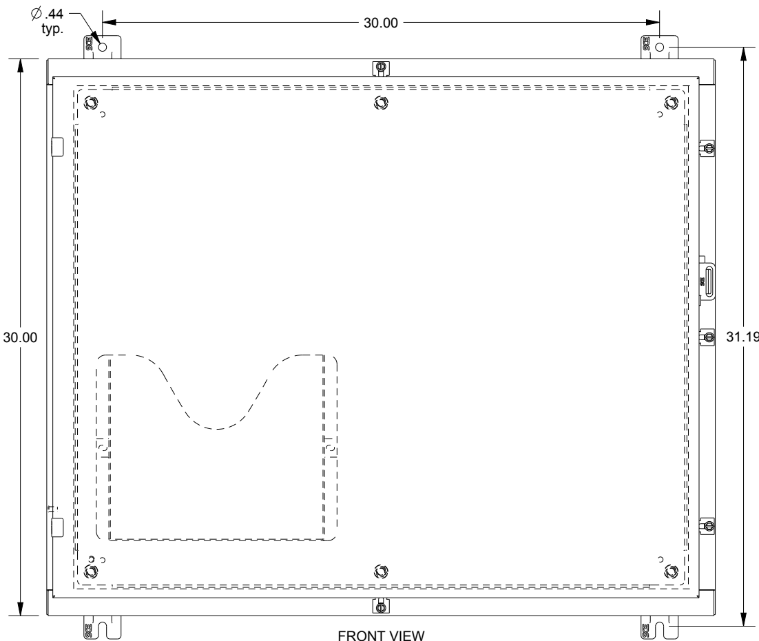
FRONT VIEW
