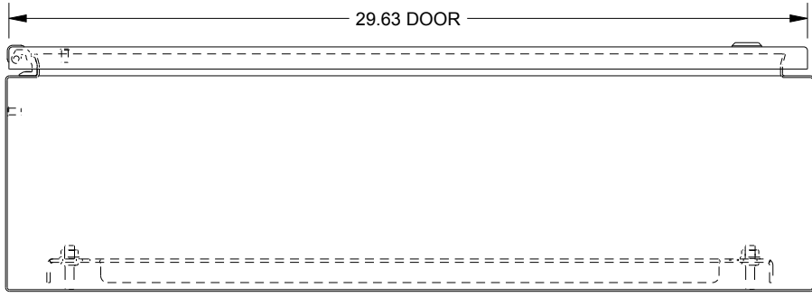
BOTTOM VIEW
