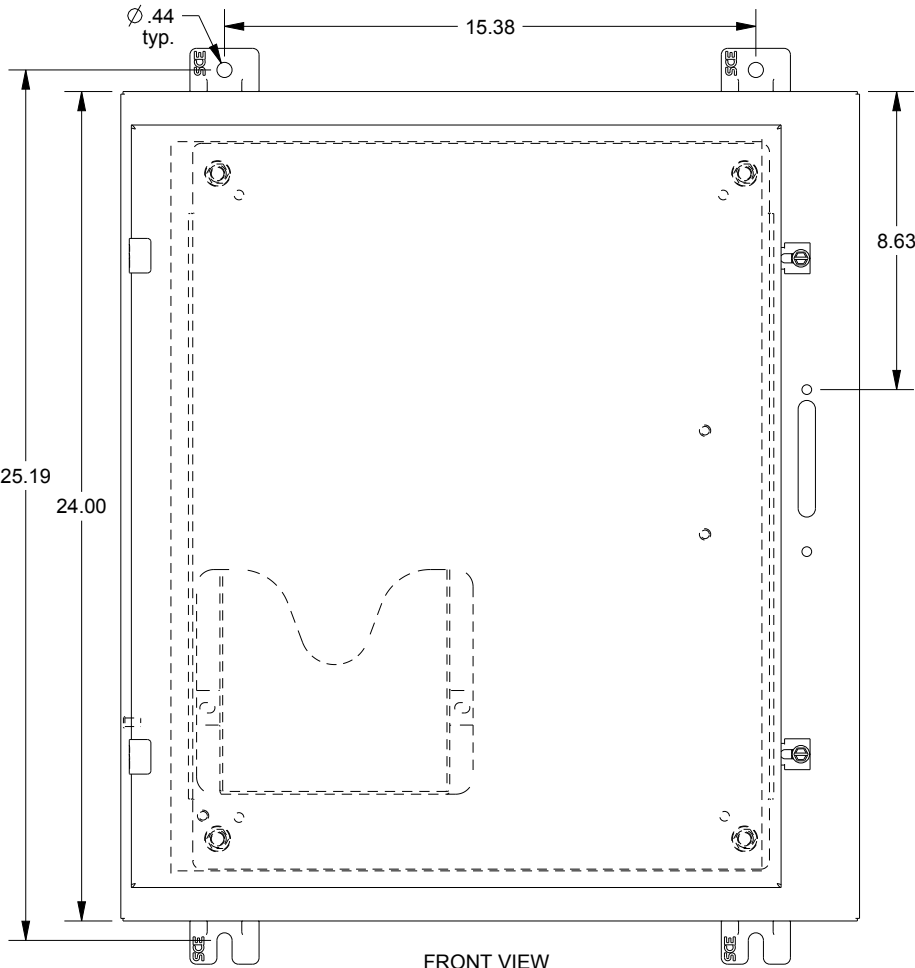
FRONT VIEW
