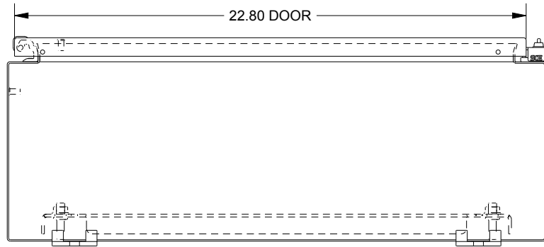
BOTTOM VIEW
