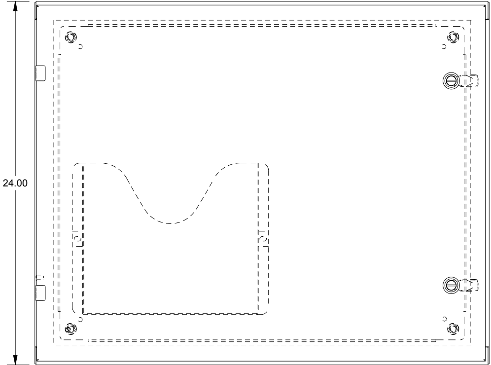
FRONT VIEW
