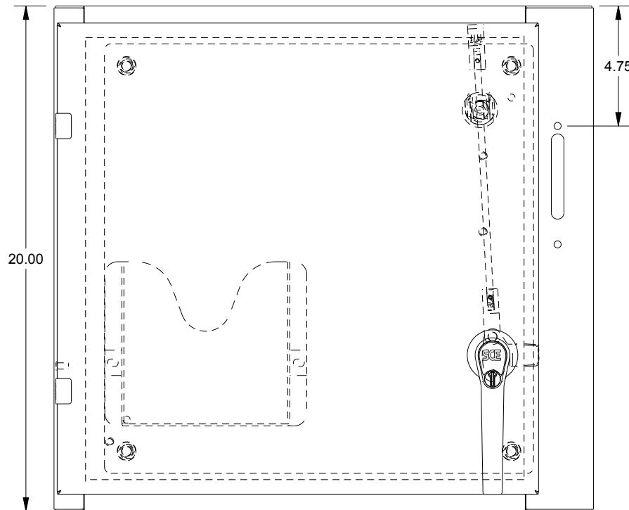
FRONT VIEW
