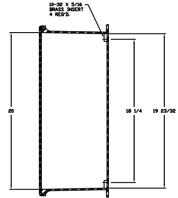
SECTION B-B
