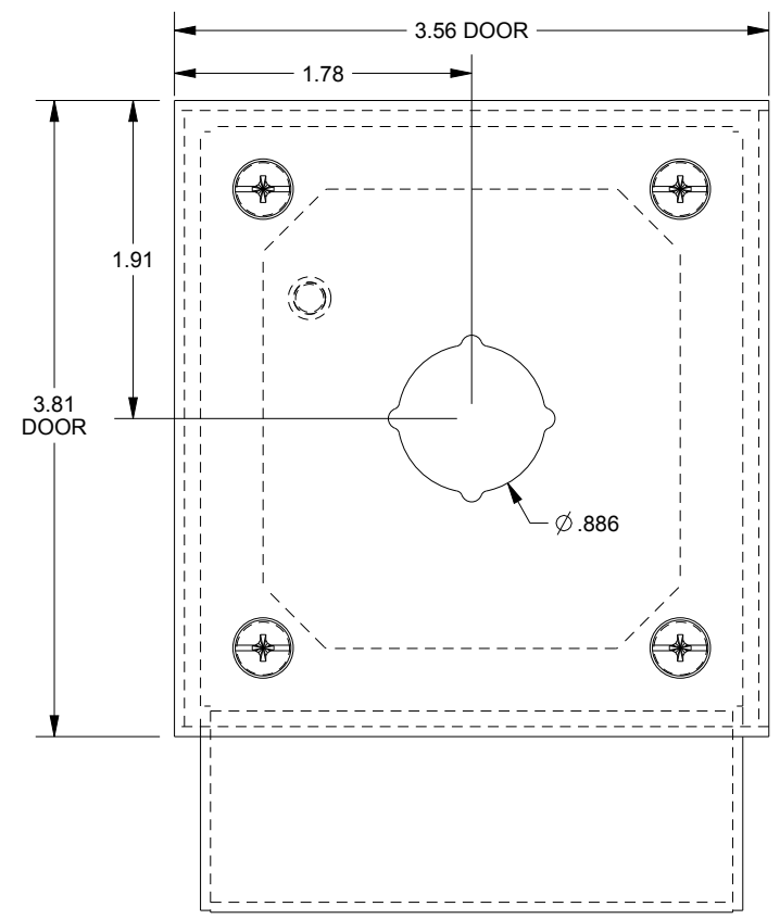
SECTION W-W
