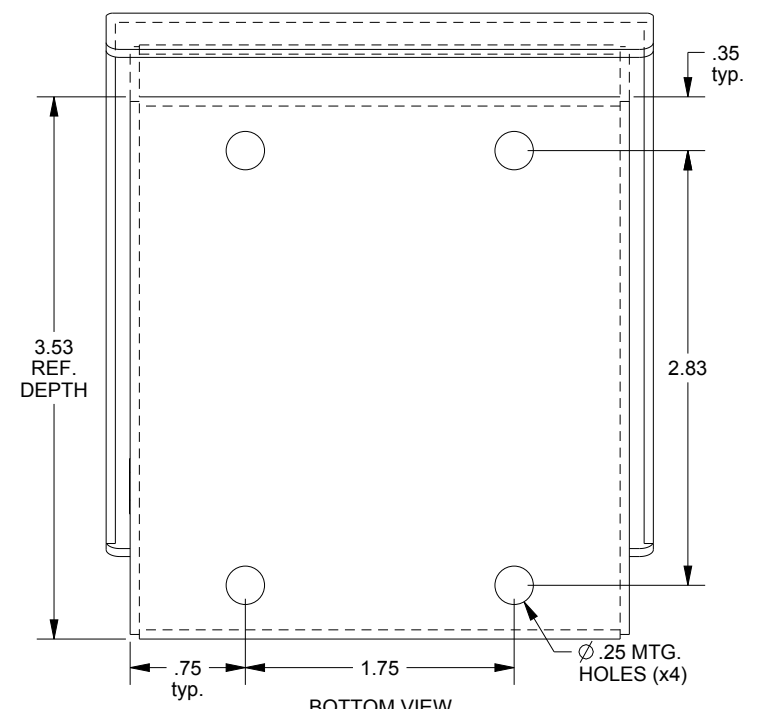
BOTTOM VIEW
