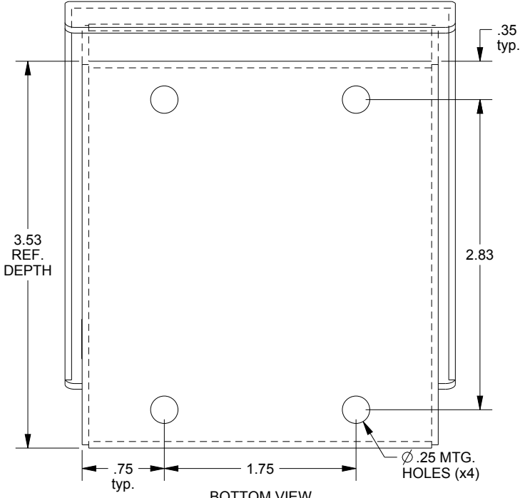
BOTTOM VIEW
